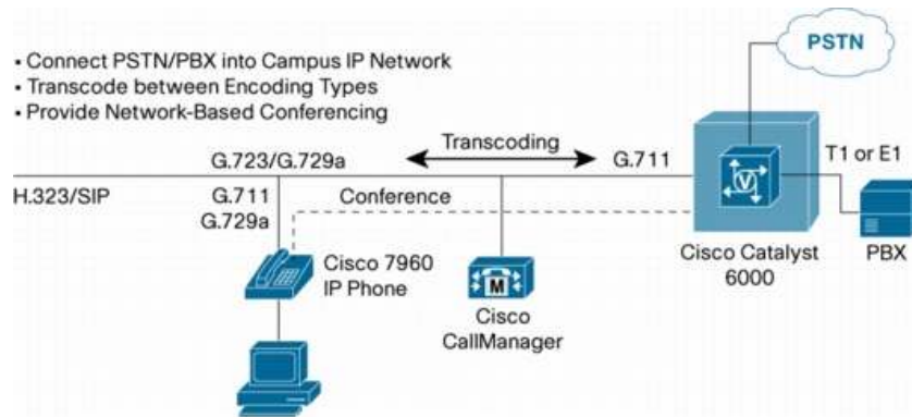
Figure 2. Cisco Unified Communication Network Deployment
